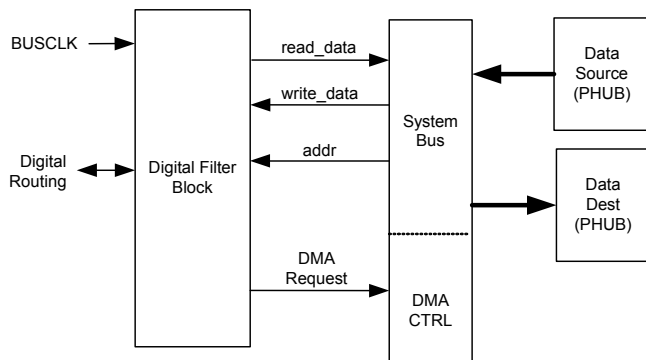
Figure 7-17. DFB Application Diagram (pwr/gnd not shown)
