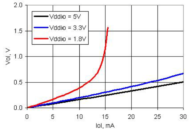
Figure 11-8. GPIO Output Low Voltage and Current
